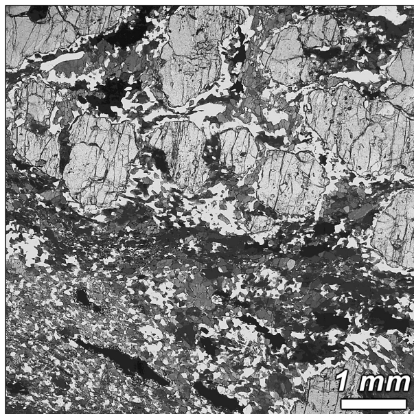
■ Fig. 15. Photomicrograph of Tisová amphibolite, Locality 3 (plane polarized light). The amphibolite assemblage is garnet, hornblende, calcic plagioclase, quartz, titanite, and ilmenite.
