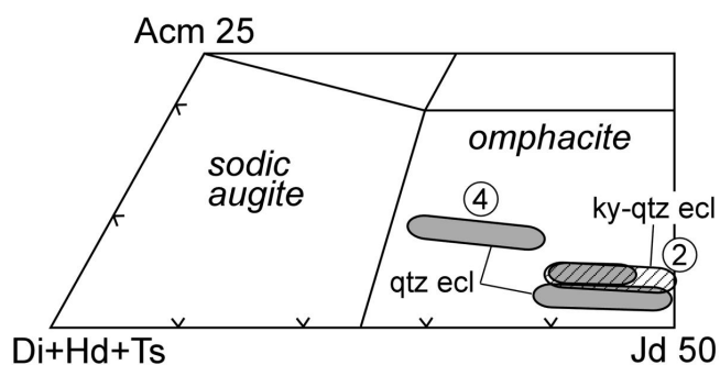
■ Fig. 5. Compositions of omphacite in MLC eclogite. Numbers: 2, omphacite in Louka kyanite-quartz eclogite; 4, omphacite in Tisová quartz eclogite.
