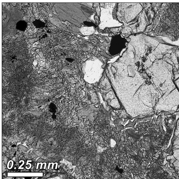
■ Fig. 14. Photomicrograph of Tisová amphibolite, Locality 3 (plane polarized light), illustrating clinopyroxene-amphibole-plagioclase symplectite after omphacite.
