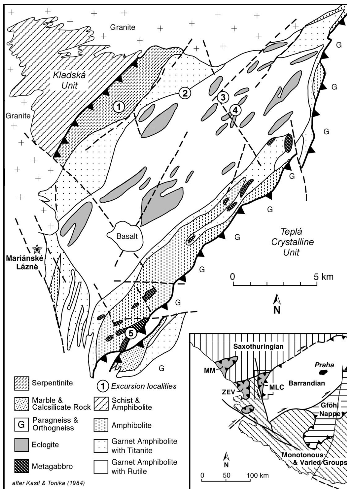
Fig. 2. Geological map of the Mariánské Lázně Complex (modified from Beard et al., 1995, after Kastl and Tonika, 1984). Excursion localities: 1, Sítiny serpentinite; 2, Louka eclogite; 3, Tisová amphibolite and feldspar veins; 4, Tisová eclogite; 5, Výškovice metagabbro.
