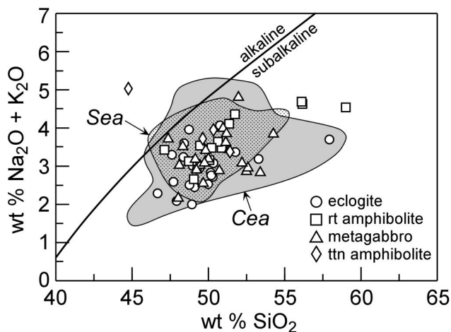
■ Fig. 6. Alkali vs. \text{SiO}_2 contents in MLC metabasic rocks; data from Beard et al., 1995; Jelínek and Štědrá, 1997. Fields: Cea, undifferentiated metabasites (Crowley et al., 2002); Sea, metagabbro (Štědrá et al., 2002).
