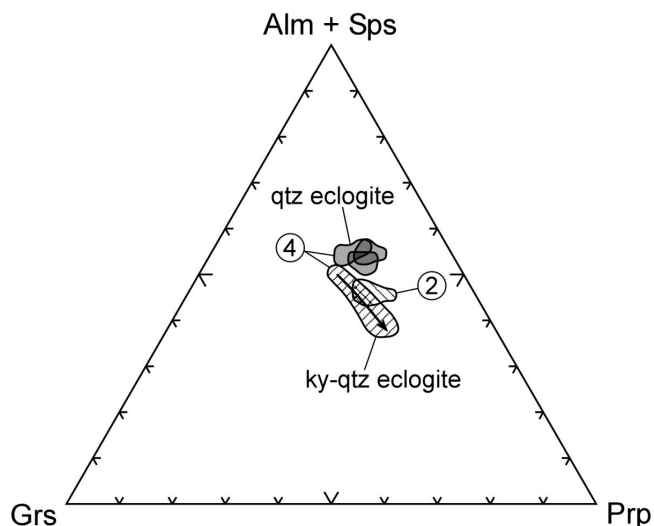
■ Fig. 4. Compositions of garnet in MLC eclogite. Numbers: 2, garnet in Louka kyanite-quartz eclogite; 4, garnet in Tisová quartz eclogite and kyanite-quartz eclogite.
