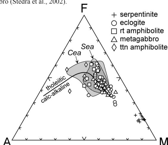
■ Fig. 7. AFM plot for MLC metabasic rocks; data from Beard et al. 1995; Jelínek and Štědrá 1997. Fields: Cea, undifferentiated metabasites (Crowley et al., 2002); Sea, metagabbro (Štědrá et al., 2002).
