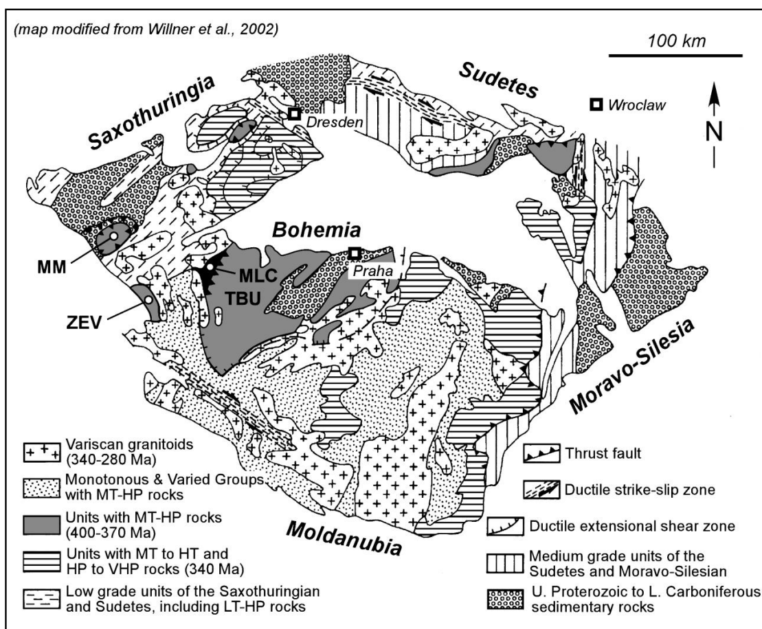
Fig. 1. Tectonostratigraphic map of the Bohemian Massif, illustrating the distribution and ages of HP and UHP metamorphism (modified after Willner et al. 2002). Abbreviations: MLC, Mariánské Lázně Complex; MM, Münchberg Massif; TBU, Teplá-Barrandian Unit; ZEV, Zone of Erbendorf-Vohenstrauss.
