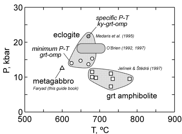
■ Fig. 11. Estimated pressure-temperature conditions for MLC eclogite, metagabbro, and garnet amphibolite. See text for methods and discussion.
