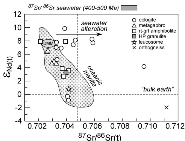
■ Fig. 9. Variation in whole-rock \epsilon_{\text{Nd}} and [^{87}\text{Sr}/^{86}\text{Sr}]_i at 540, 500, and 370 Ma (see text) for MLC metabasic and other rock types. Data from Beard et al., 1995; Timmermann et al., 2004.
